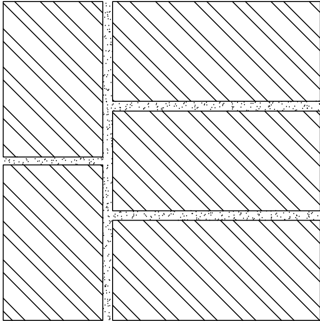
English bond
