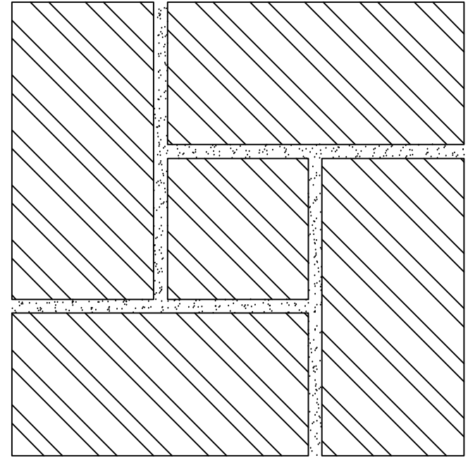
Flemish bond
